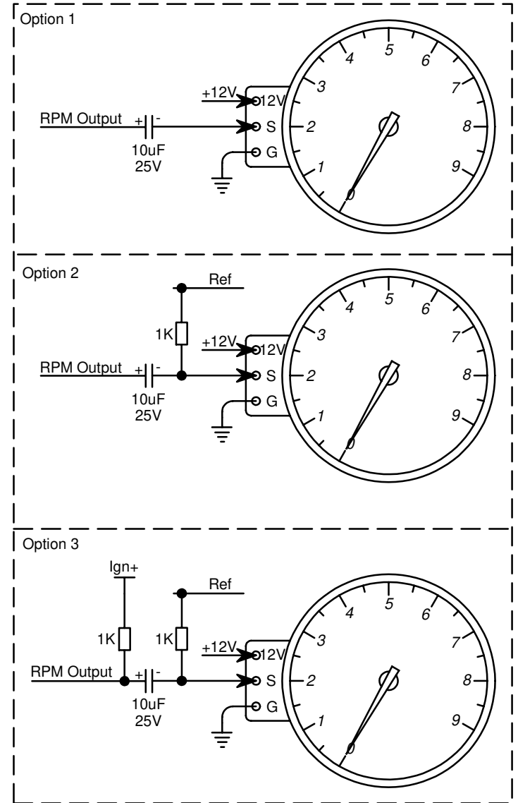
Magnetic Pickup Tachometers
