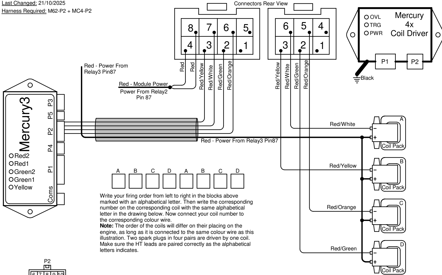
Harness Pin View
